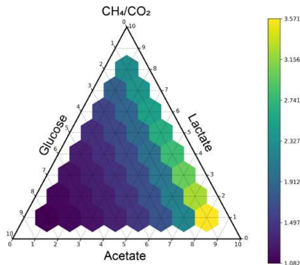
Fig. 2. Biogas composition as a function of the relative concentrations of acetate, lactate, and glucose in the anaerobic digestion feedstock. The colored bar shows the ratio of \text{CH}_4 to \text{CO}_2 from 3.6 (78% \text{CH}_4 ) to 1 (50% \text{CH}_4 ).
