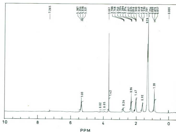
Fig.1. 1 H NMR of biodiesel derived from the waste fish oil
