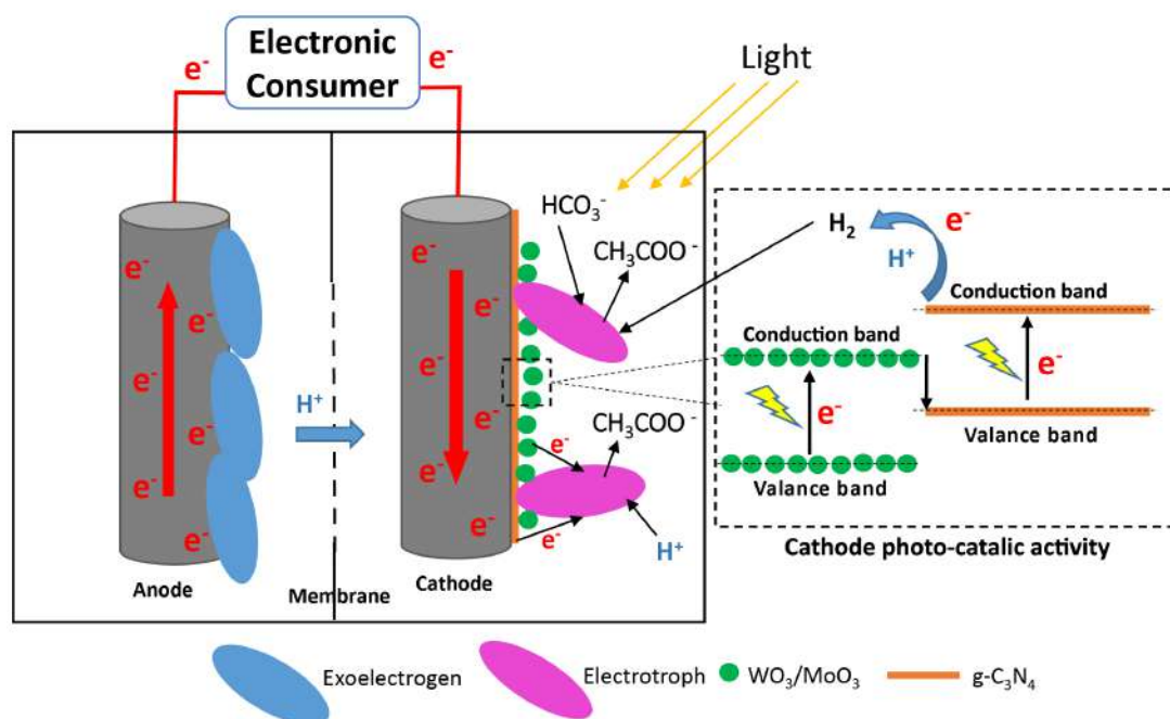
Fig. 4. Effect of cathode modification with \text{WO}_3 and \text{MoO}_3 nanoparticles (possessing photocatalytic activity) on the system performance, i.e., promoting hydrogen evolution and the consequent increased acetate production by the electrotroph Serratia marcescens . Adapted from Cai et al. (2020b).
