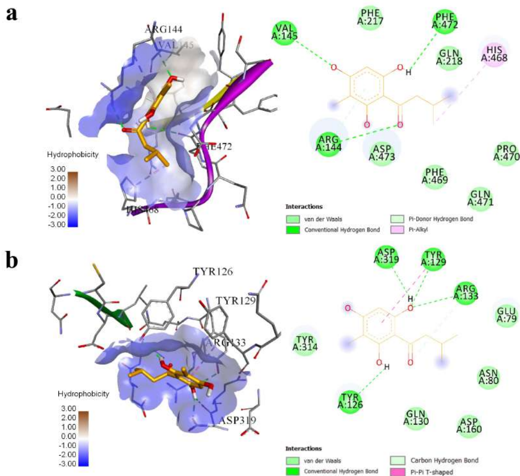
Fig. 4. 3D mode and 2D interaction of non-covalent interaction of 1-butane-3-methyl-1-(2,4,6-trihydroxy-3-methylphenyl)- with (a) AKT (3QKK) and (b) ERK2 (6NBS).
