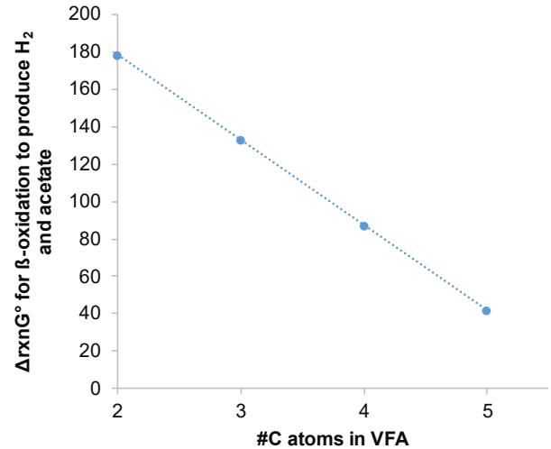
Fig. 2. The plot of \Delta_{rxn}G^\circ(25^\circ\text{C}) for \beta -oxidation of VFAs to produce H 2 (aq), CO 2 (aq), and acetate(aq), i.e., the reactions presented in Equations 13-19. structures
