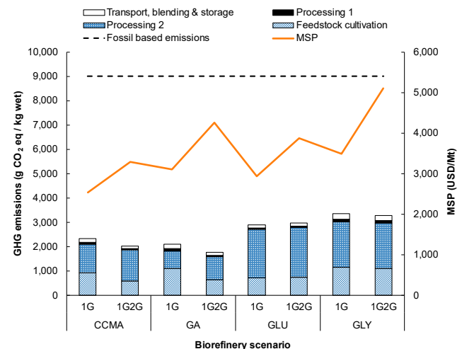
Fig. 7. GHG emissions associated with the various ADA biorefinery scenarios compared to the corresponding minimum selling prices (MSPs) and the fossil-based ADA emissions for the United States in 2017 ( Flederbach and Winch, 2019 ) in terms of g CO 2 eq/kg wet product.
