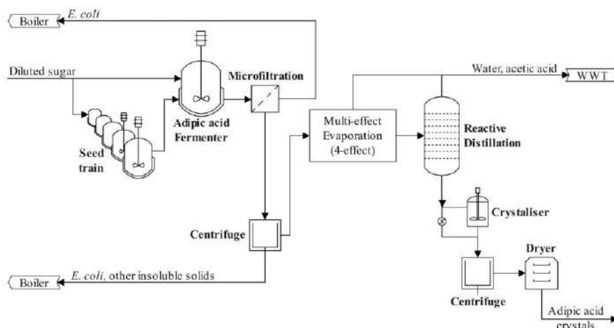
Fig. 3. Adipic Simplified process flow diagram of the direct adipic acid pathway scenario.
